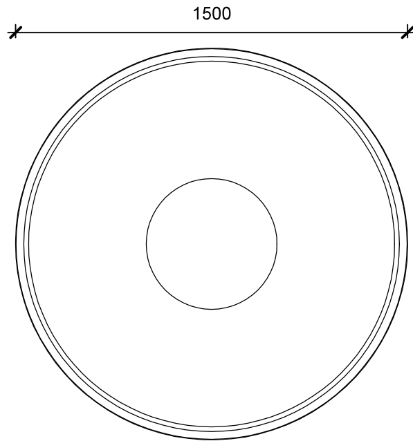
1 Plan View 1 : 20
